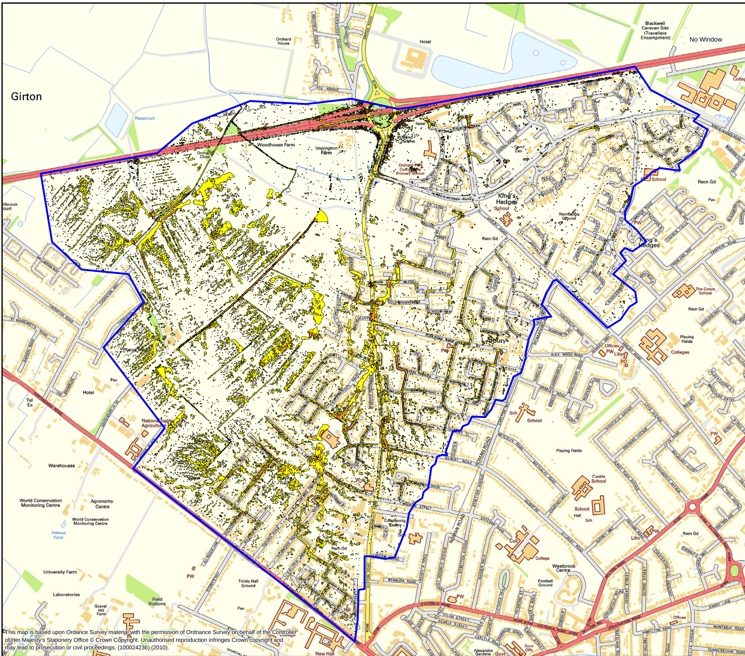
FIGURE F35 1.5% AEP "DO MINIMUM" PLUVIAL MODELLING MAXIMUM VELOCITY - KING'S HEDGES AND ARBURY
